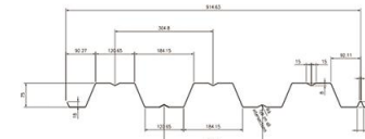
3" VLI Composite Deck Coil Width ~ 1270.8 mm
